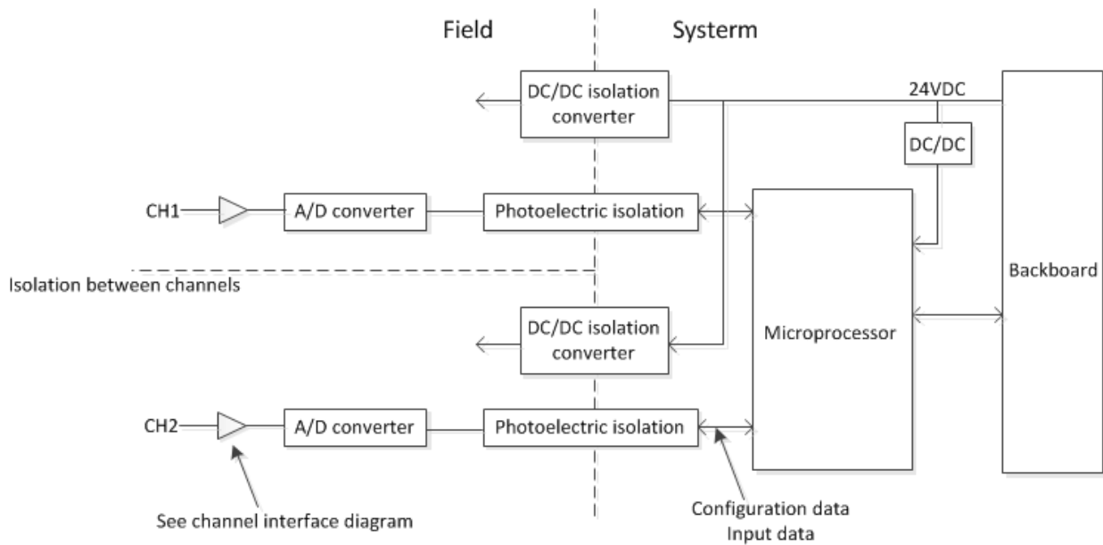
Internal Structure Block Diagram of LK442
