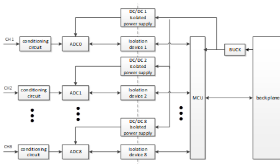
Internal structure block diagram of LK432 module
