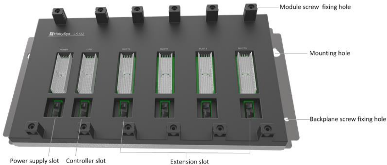
LK132 Backplane Schematic Diagram
