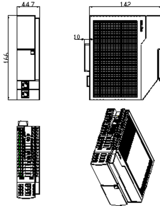
LK241 Module Dimension
