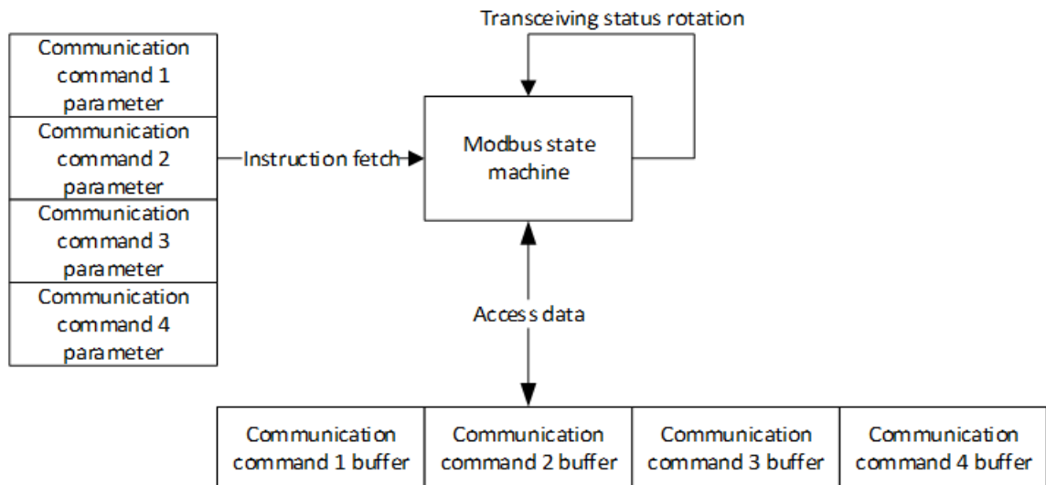
Serial Port Module Communication Command Polling Schematic Diagram
