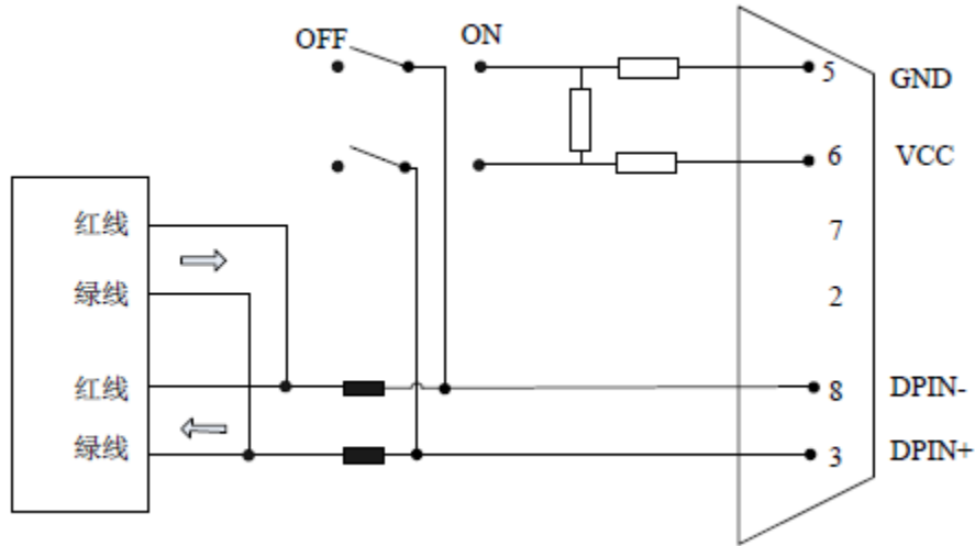
LKA107 Schematic Diagram
