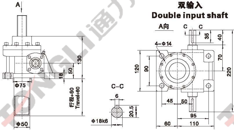
S型(牙口式) S shape(bolt model)
