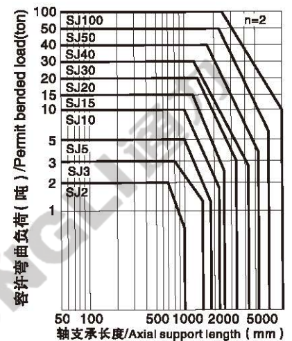
底座固定—轴端固定或支撑 Fixed pedestal—Fixed axle head or axle head support
