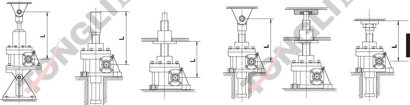
底座支承—轴端支承 Pedestal support—Axle head support
