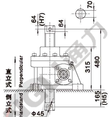
R型(平头式) R shape(flat axle head model)
