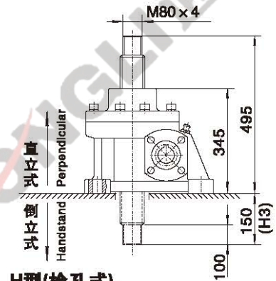
H型(栓孔式) H shape(keyhole model)
