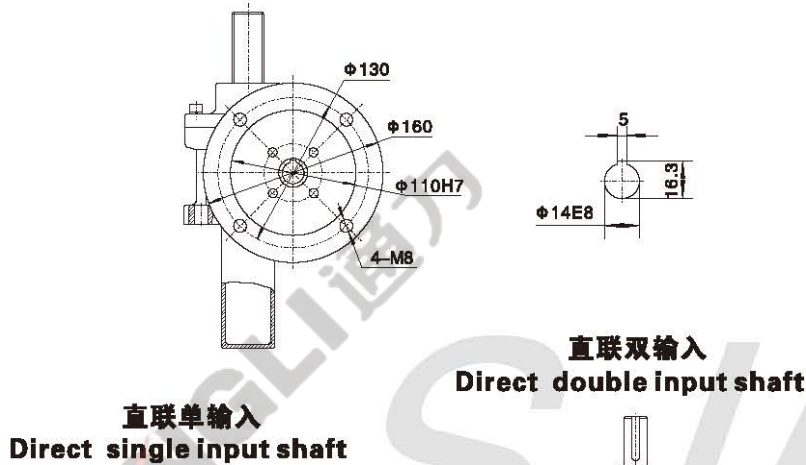
H型(栓孔式) H shape(keyhole model)
