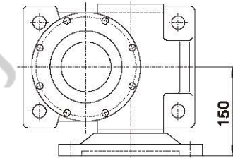
直联单输入 Direct single input shaft
