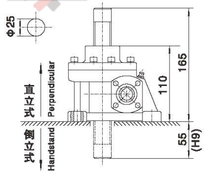
T型(顶板式)/T shape(roof model)
