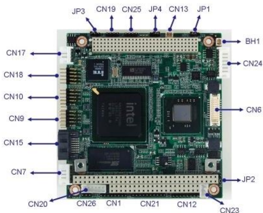
Figure 2.1 Connectors (component side)
